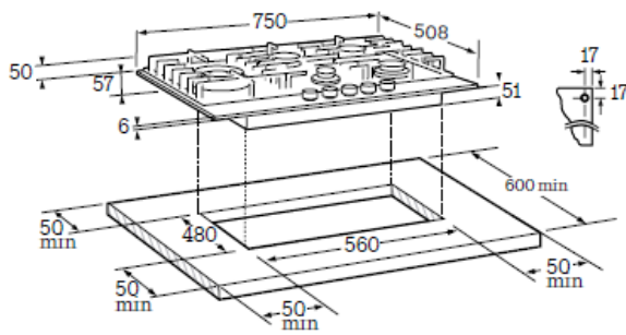
GAS HOB 75 cm SOTG1730B | SOTG1730W
