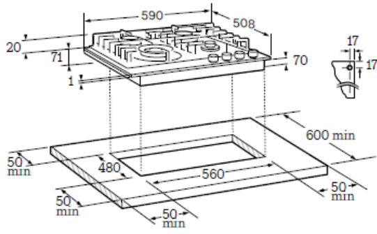
GAS HOB 60 cm SOTE1630X
