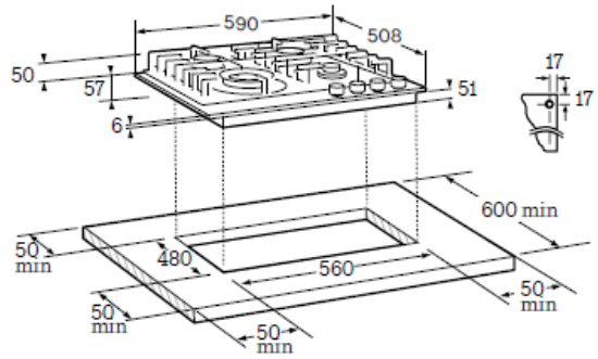
GAS HOB 60 cm SOTG1630B | SOTG1630W
