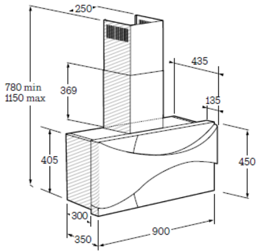
VERTICAL WALL HOOD SOHV1940X
