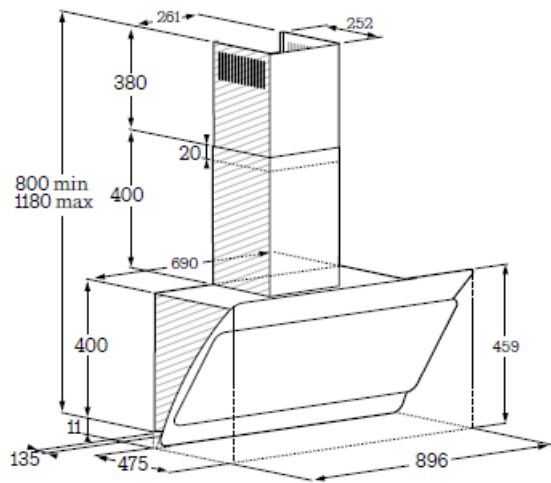
INCLINED WALL HOOD SOHV1920B
