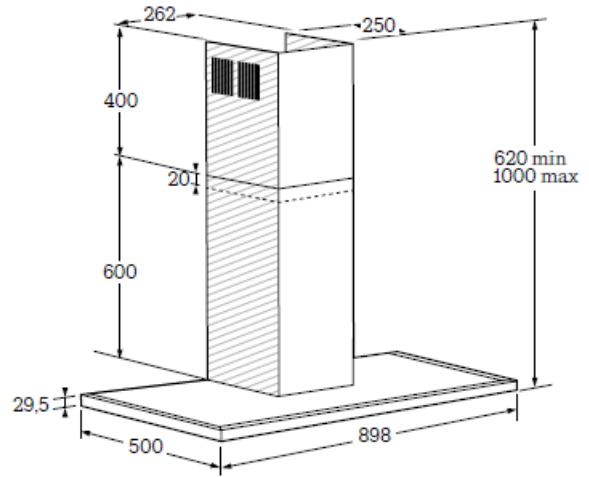
BOX WALL HOOD SOHB1930X
