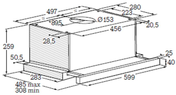
TELESCOPIC HOOD 60 cm SOHT1610X
