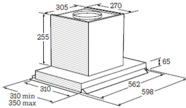
FILTER UNIT 60 cm SOHG1620X
