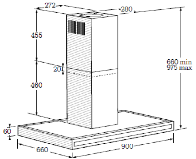
BOX ISLAND HOOD SOHI1910X
