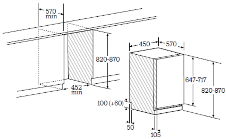
DISHWASHER 45 cm SODV1410F
